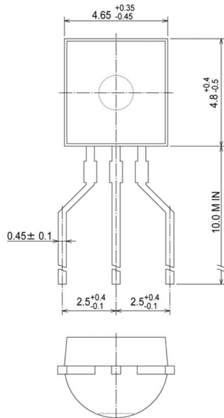
TO-92
